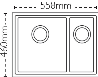
Bowl Depth. Main Bowl 205mm Half Bowl 178mm
