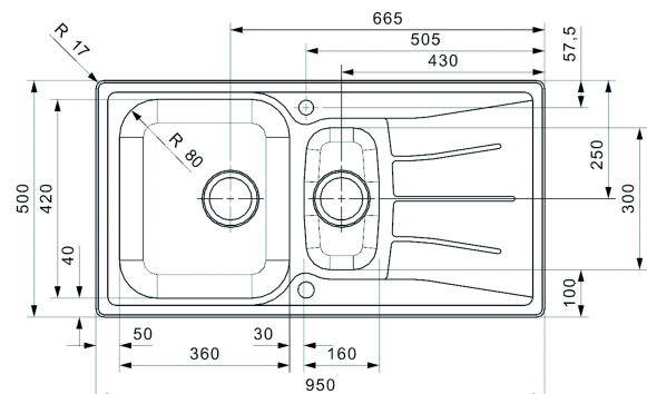
Bowl Depth Main Bowl 160mm - Half Bowl 130mm
