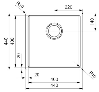
Bowl Depth 200mm
