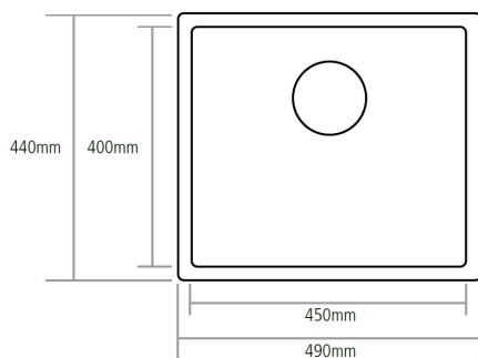
Bowl Depth 200mm
