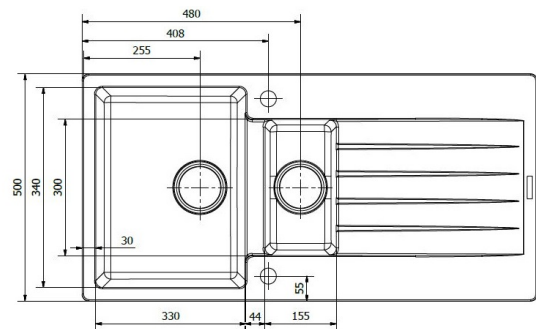
Bowl Depth Main Bowl 200mm - Half Bowl 140mm
