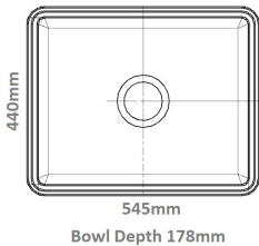
Reginox Mataro Single bowl undermount sink. MATARO / £143.57 Available in white Cabinet size: 600mm Min SUITABLE FOR WASTE DISPOSAL UNIT- YES
