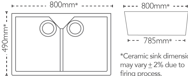
Sink 220mm High - Bowl depth 200mm
