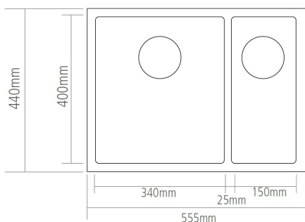
Bowl Depth Main Bowl 200mm - Half Bowl 135mm
