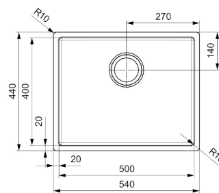
Gunmetal Effect MIAMI50/GM / £327.29
