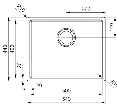
Bowl Depth 200mm
