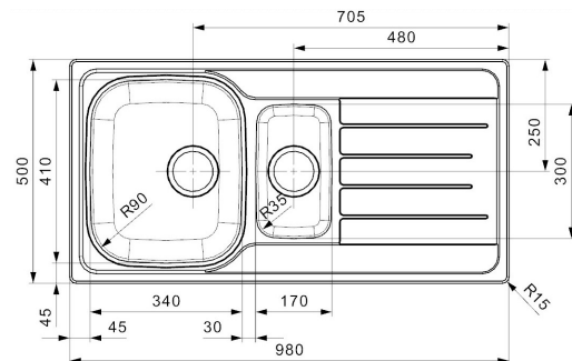
Depth Main Bowl 170mm - Half Bowl 128mm
