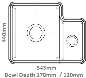
Reginox Tuscany 1.5 bowl undermount sink. TUSCANY / £170.36 Available in white with R/H half bowl / drainer only Cabinet size: 600mm Min SUITABLE FOR WASTE DISPOSAL UNIT- YES
