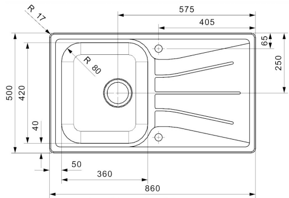
Bowl Depth 160mm
