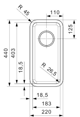
Bowl Depth 180mm
