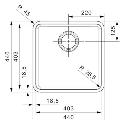
Bowl Depth 180mm
