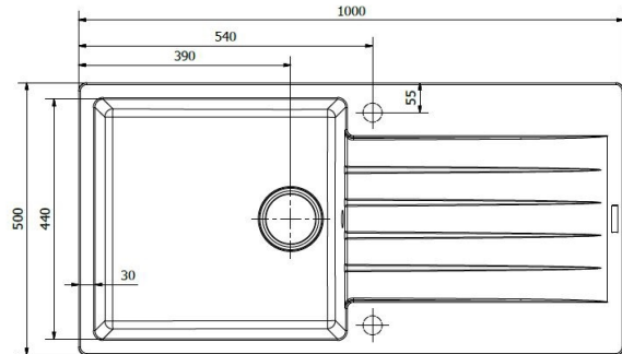
Bowl Depth 200mm
