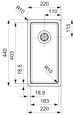
Bowl Depth 145mm
