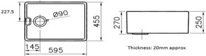
Reginox ceramic belfast sink. BELFAST / £121.29 Available in white To suit 460mm High x 600mm Wide Cabinet SUITABLE FOR WASTE DISPOSAL UNIT- NO
