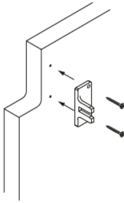
Step 1. Attach quick fix brackets to routed cabinet gables using screws.
