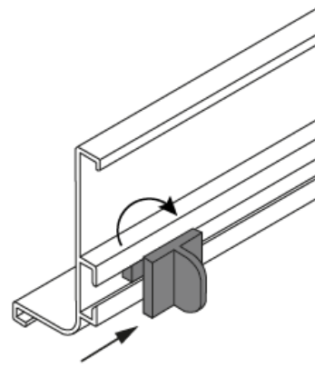
Step 2. Slide the connectors into the back of the profile and turn 90 degrees.
