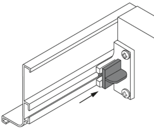
Step 1. Attach quick fix brackets to routed cabinet gables using screws.
